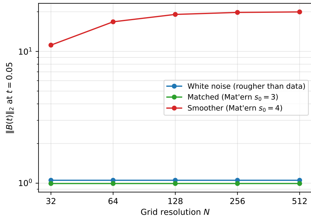
Drift Lipschitz vs. resolution at t = 0.05
