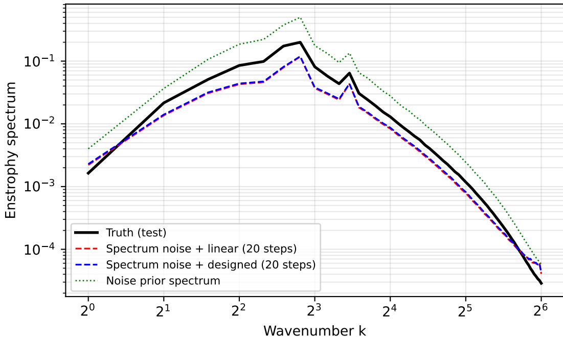
NS 128x128: spectrum noise prior, \lambda^* = 5.008e-01
