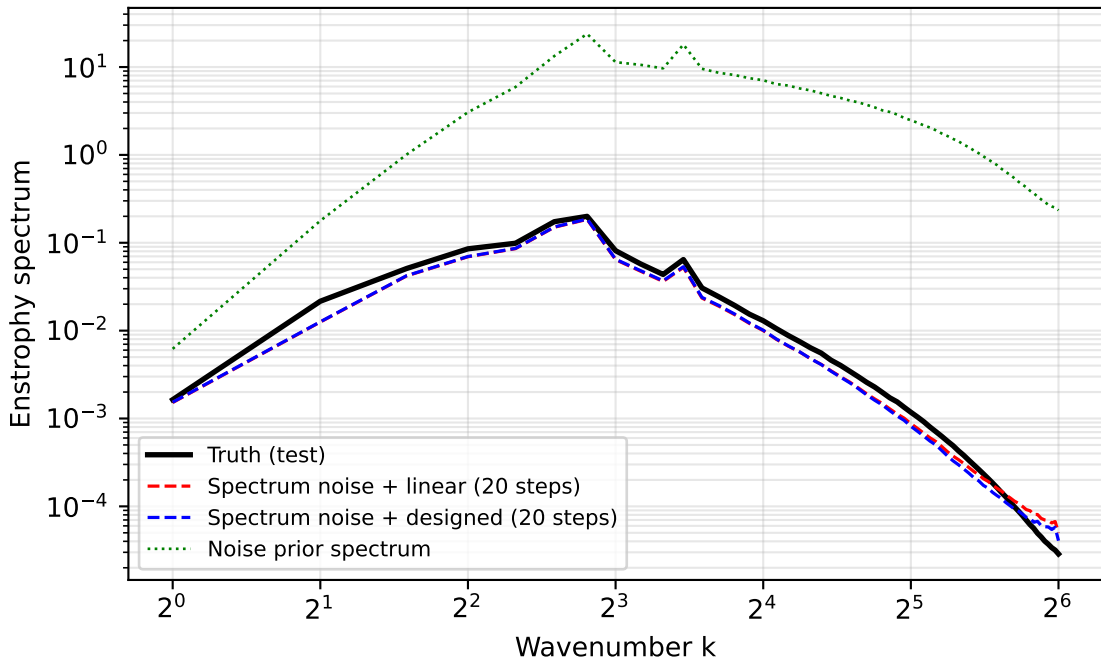
NS 128x128: spectrum noise prior, \lambda^* = 1.226e-04
