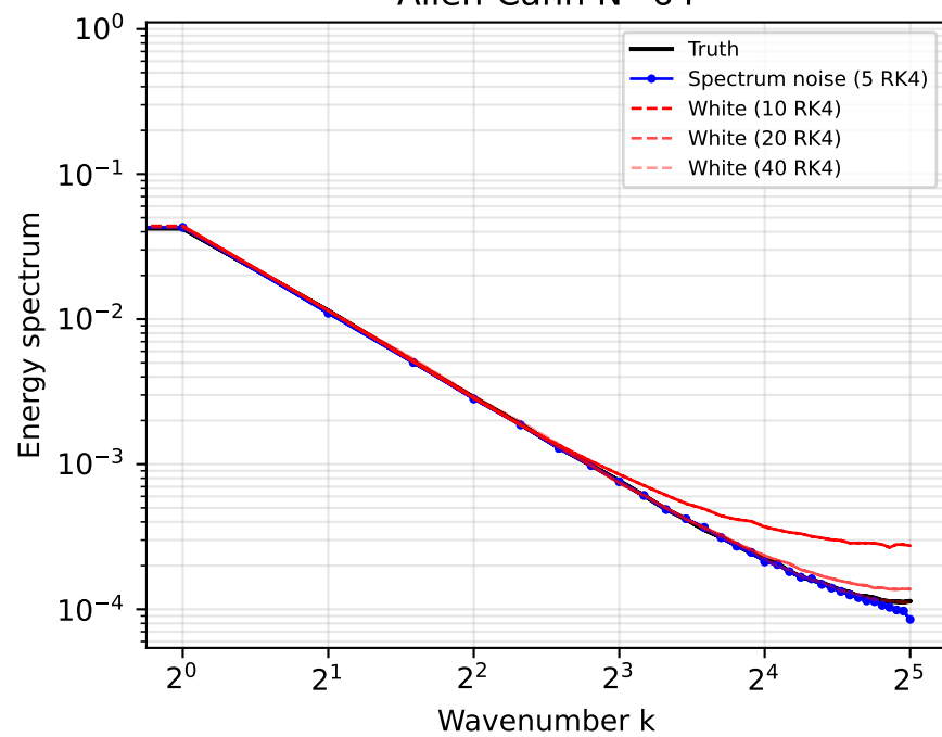
Allen-Cahn N=64
