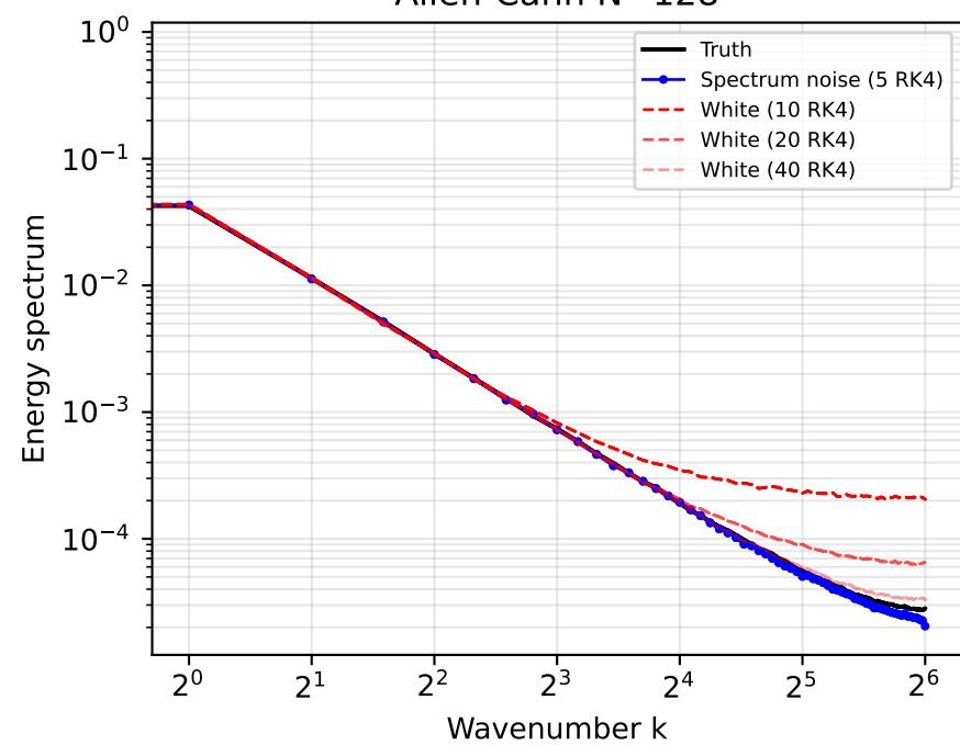
Allen-Cahn N=128
