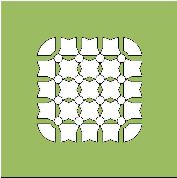
Plane Gets "Chewed Up" Using Thermal Relief Vias
