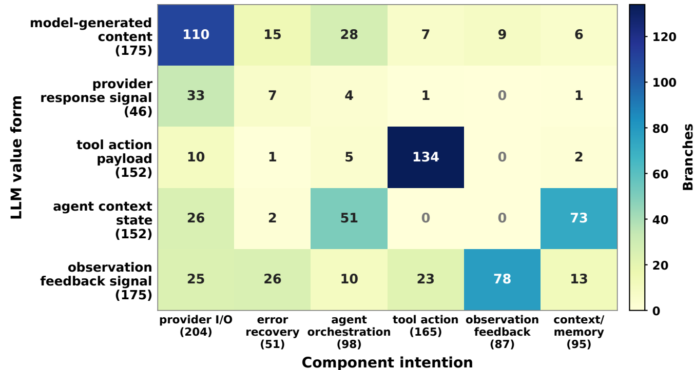
LLM value form to component intention
