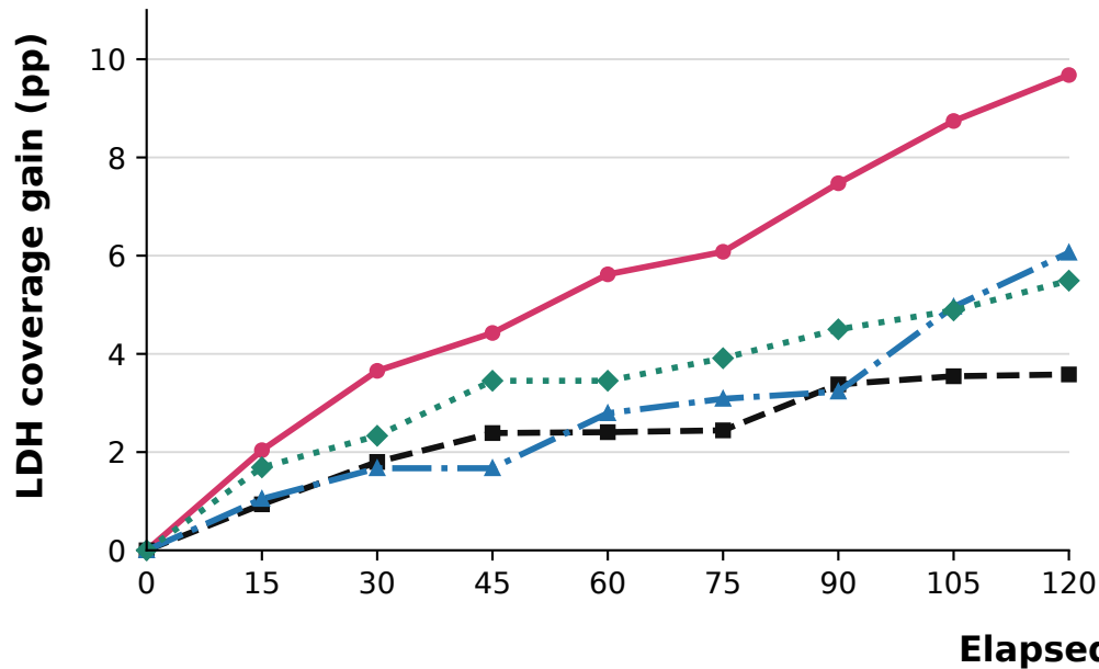
Line coverage
