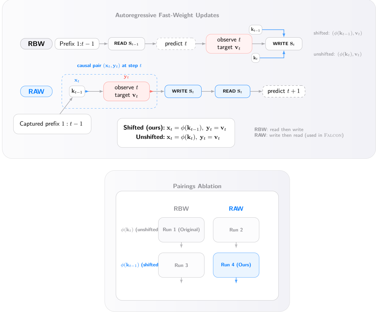
Figure 7 Formal timing conventions. Above: We explicitly distinguish read-before-write (RBW) and read-after-write (RAW) autoregressive fast-weight updates. Under the RAW convention used in FALCON, the causally aligned training pair at step t is (\phi(\mathbf{k}_{t-1}), \mathbf{v}_t) , i.e., a prefix write feature paired with the newly revealed target. Below: A 2 \times 2 design over timing convention \{\text{RBW}, \text{RAW}\} and write pairing \{\text{same-step, shifted}\} separates causal timing from mere index shifting; in the kernelized setting these pairings are understood in write-feature space, i.e. \{\phi(\mathbf{k}_t), \phi(\mathbf{k}_{t-1})\} .
