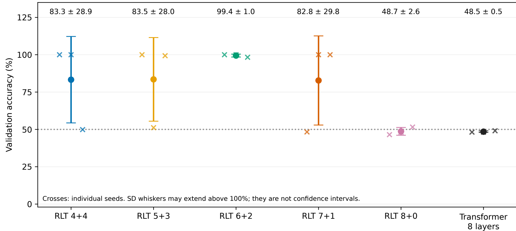
Parity at step 500: mean \pm sample SD across seeds 42, 43, 44
