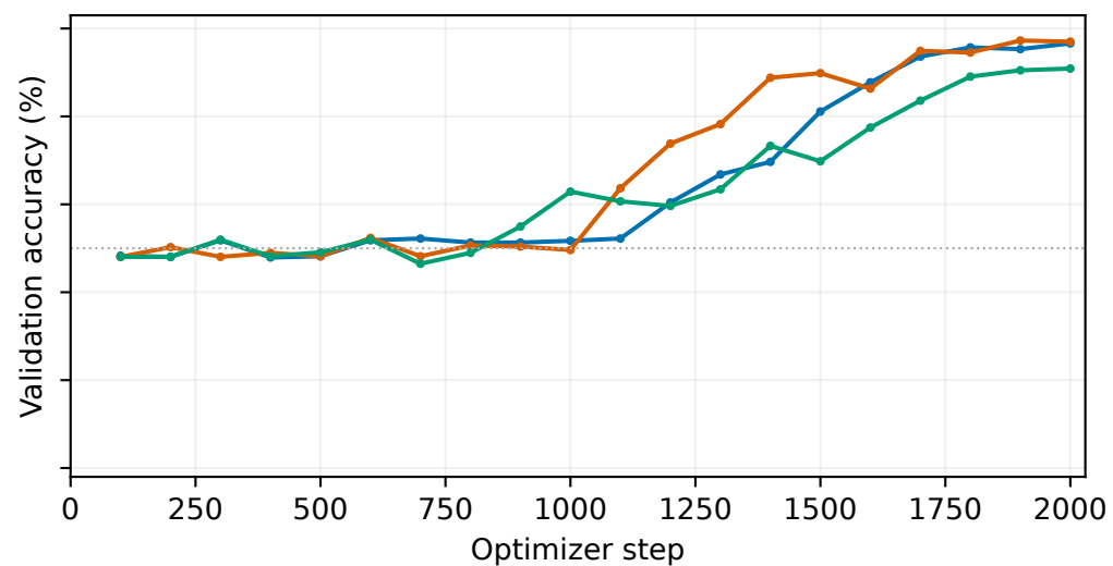
Transformer 8
