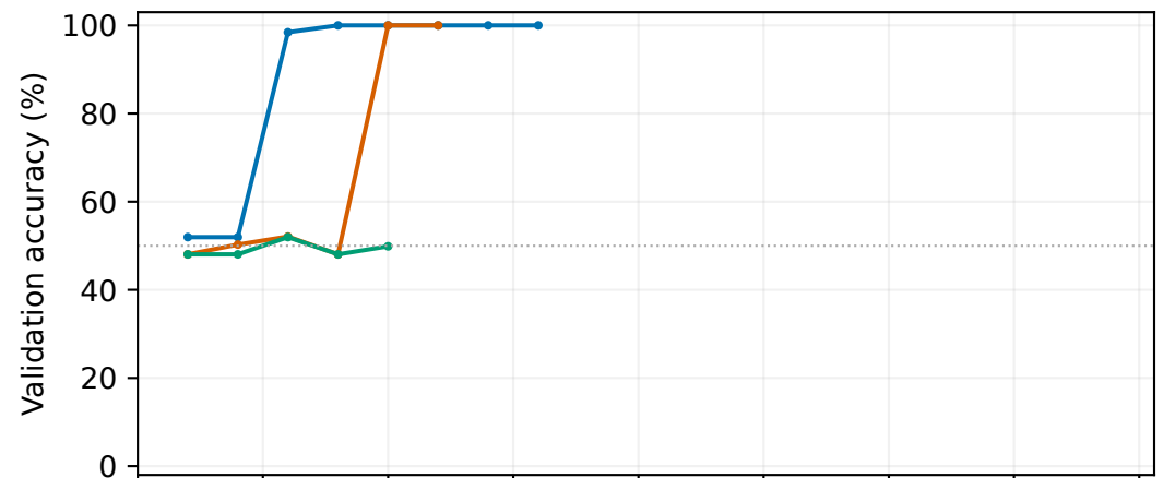
RLT 6+2
