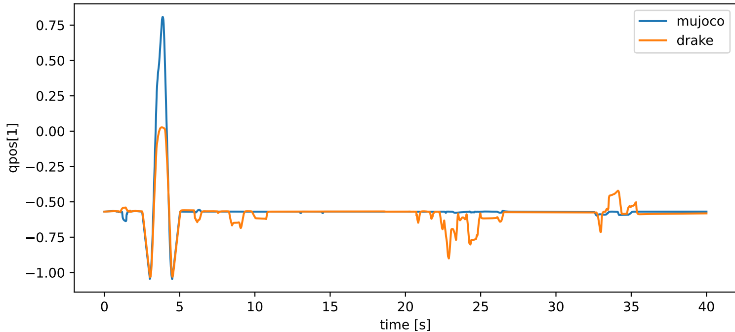
grasp_reorient: qpos[1] vs time
