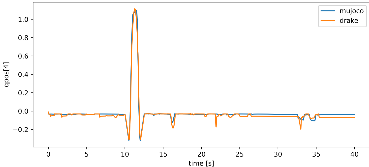
grasp_reorient: qpos[4] vs time
