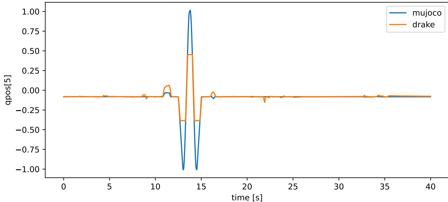
grasp_reorient: qpos[5] vs time
