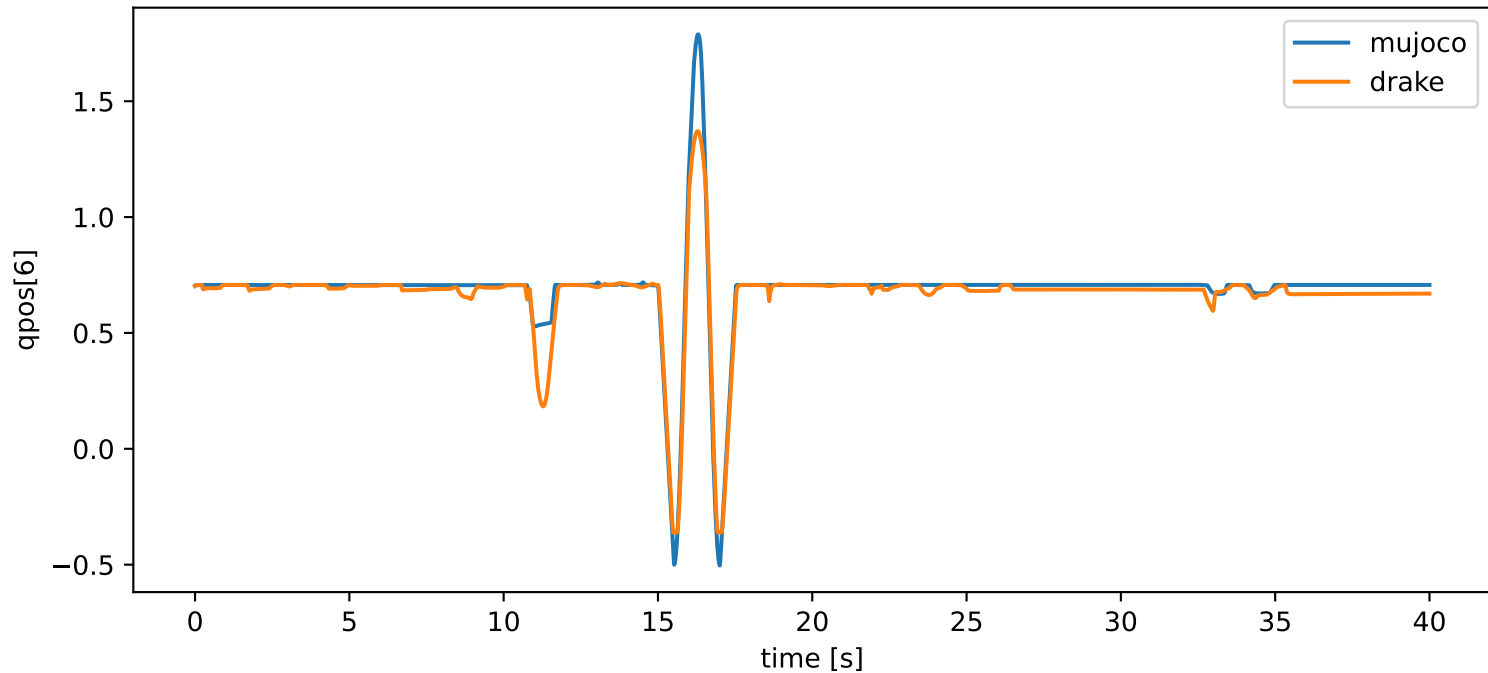
grasp_reorient: qpos[6] vs time
