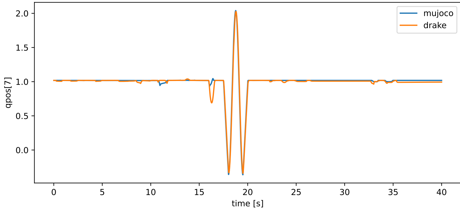
grasp_reorient: qpos[7] vs time
