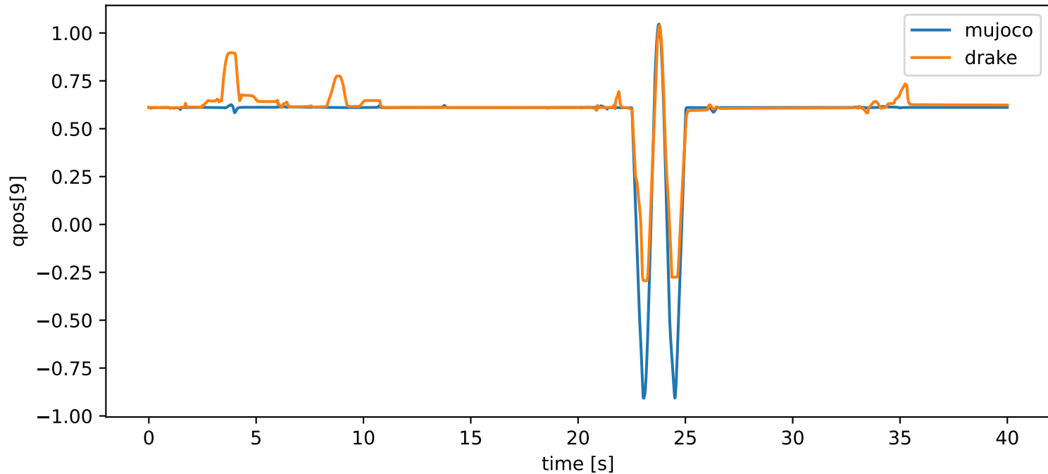
grasp_reorient: qpos[9] vs time
