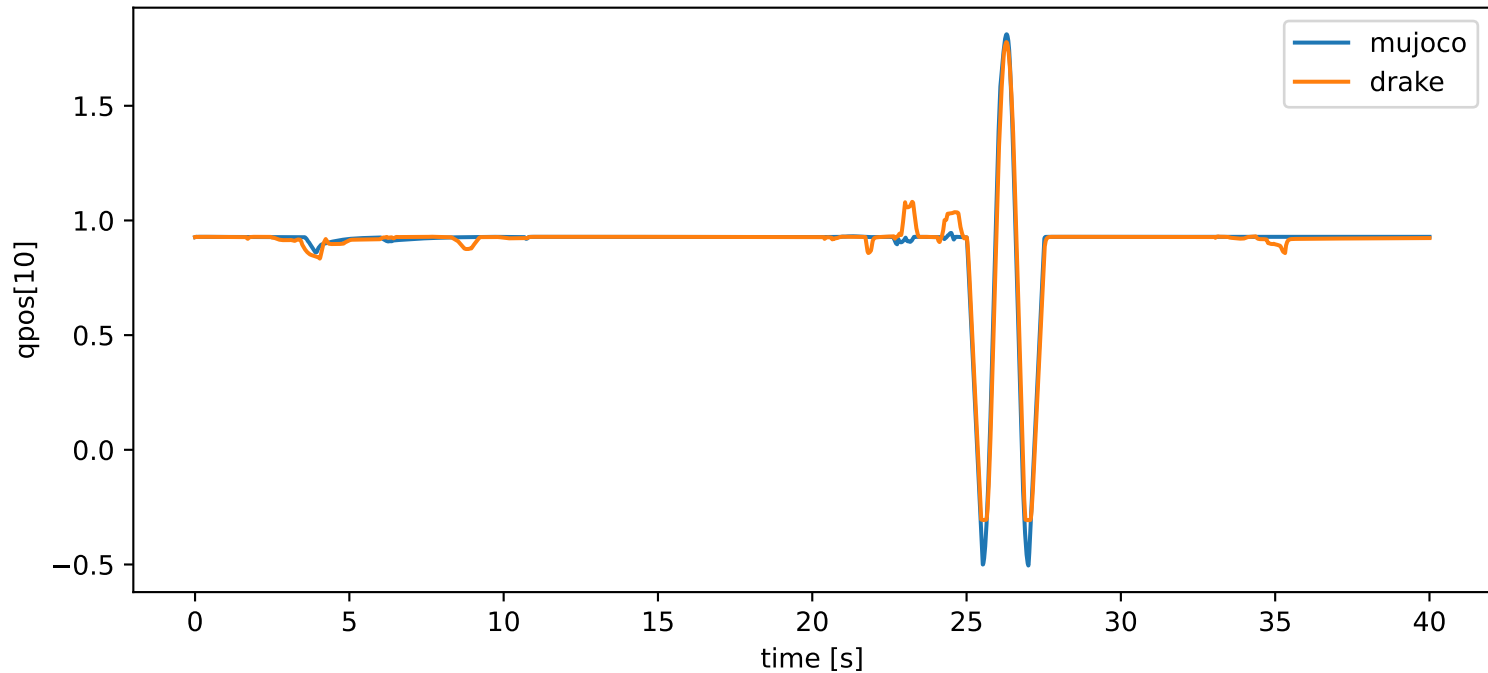
grasp_reorient: qpos[10] vs time
