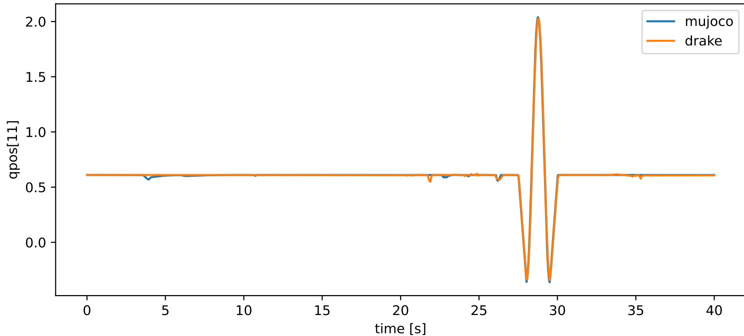
grasp_reorient: qpos[11] vs time
