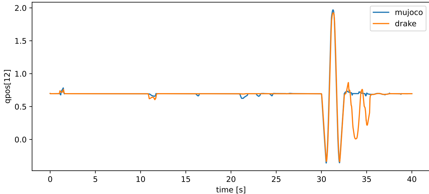
grasp_reorient: qpos[12] vs time
