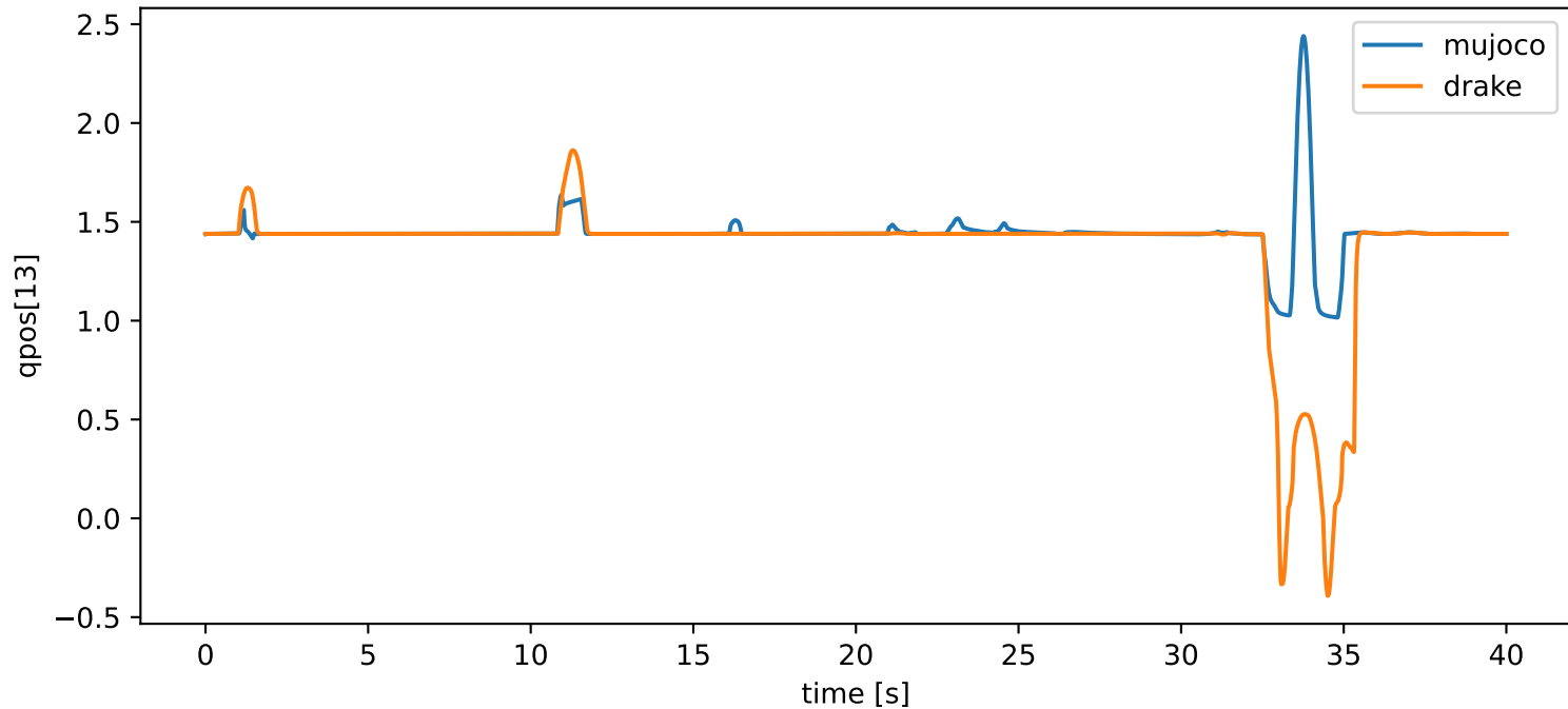
grasp_reorient: qpos[13] vs time
