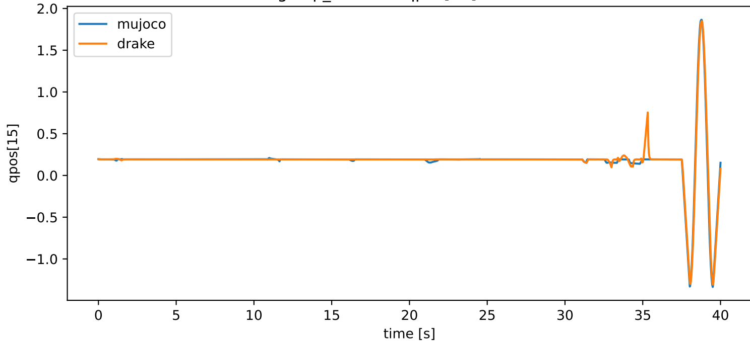
grasp_reorient: qpos[15] vs time
