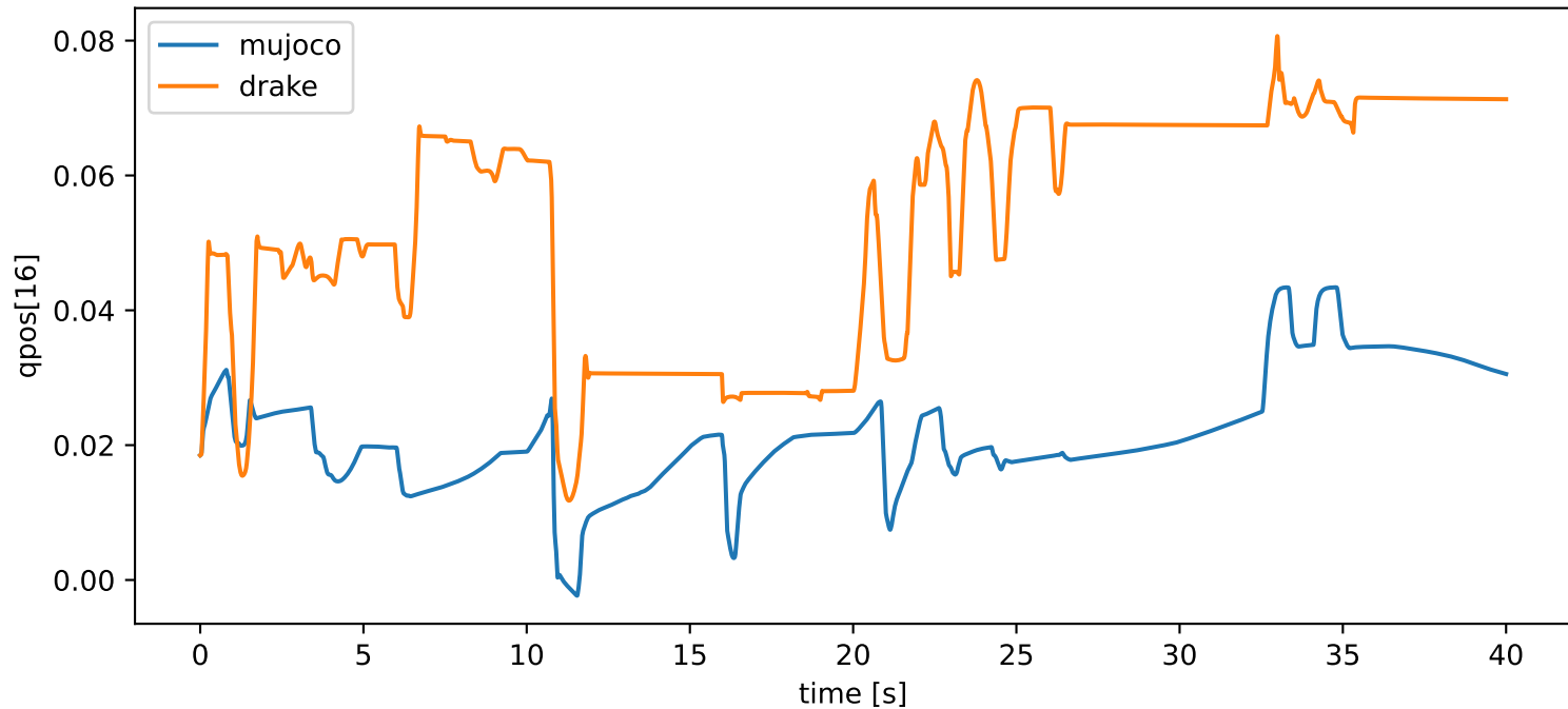
grasp_reorient: qpos[16] vs time
