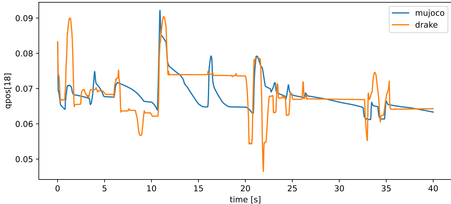
grasp_reorient: qpos[18] vs time
