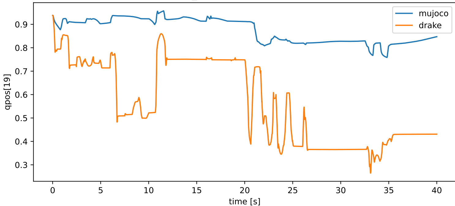
grasp_reorient: qpos[19] vs time
