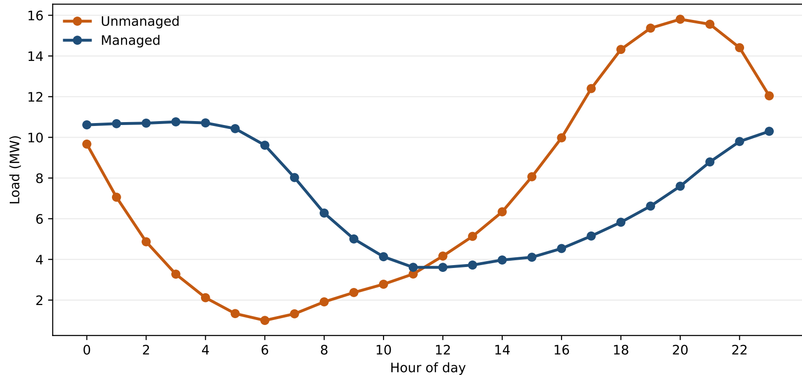
2027 baseline adoption-scaled hourly charging load
