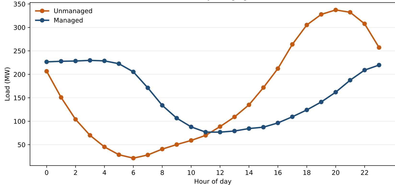
Full-EV hourly charging load
