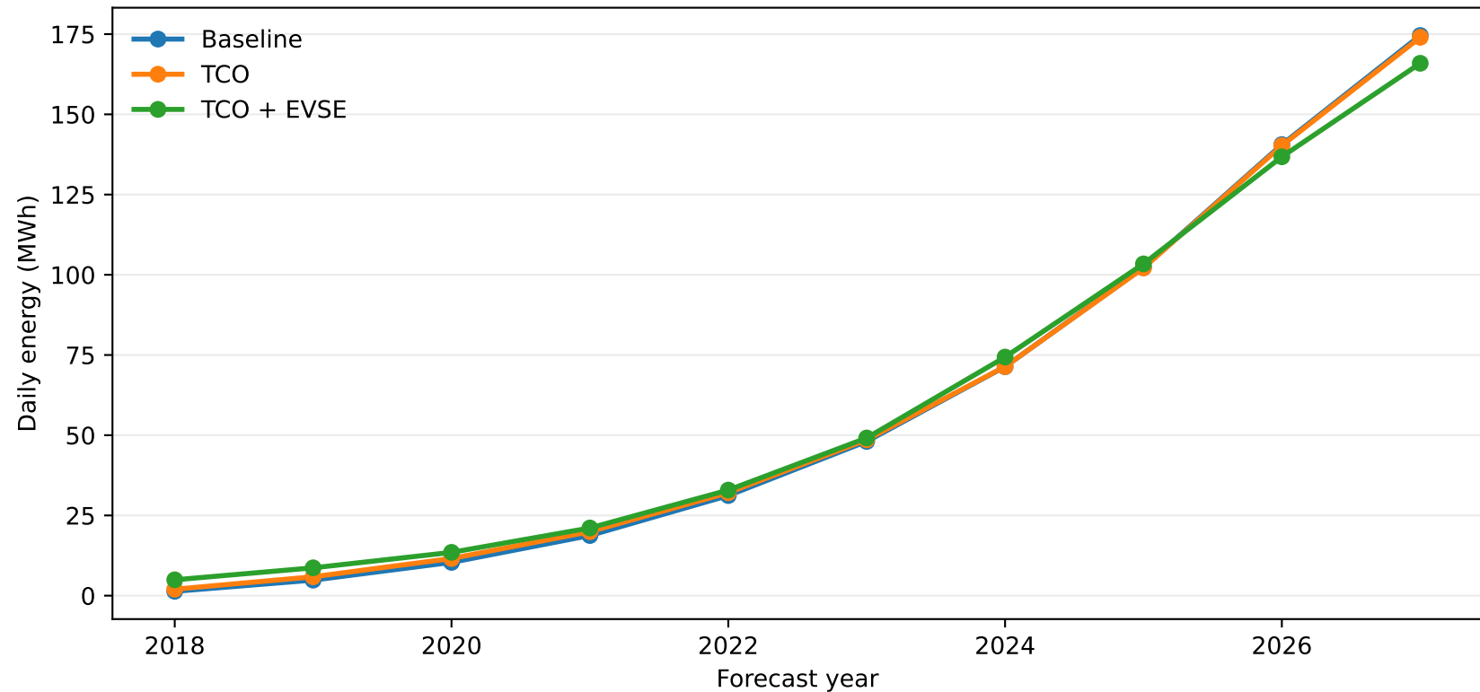
Adoption-scaled daily charging energy
