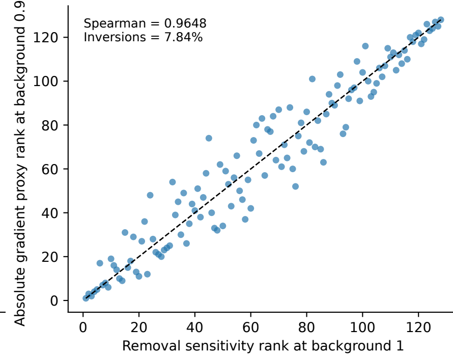
(f) Counterexample 3
