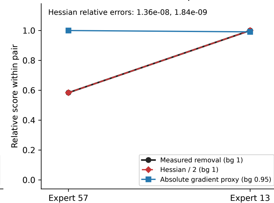
(f) Counterexample 3
