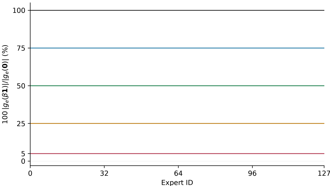
All experts scaled together: measured partial gradients, layer 0, 32 GQA samples L2 (128/128 valid ratios)
