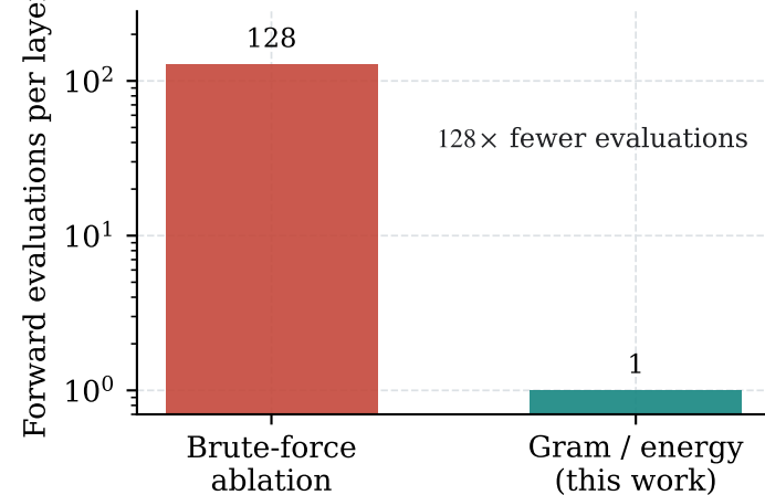
(c) Cost of the same exact score
