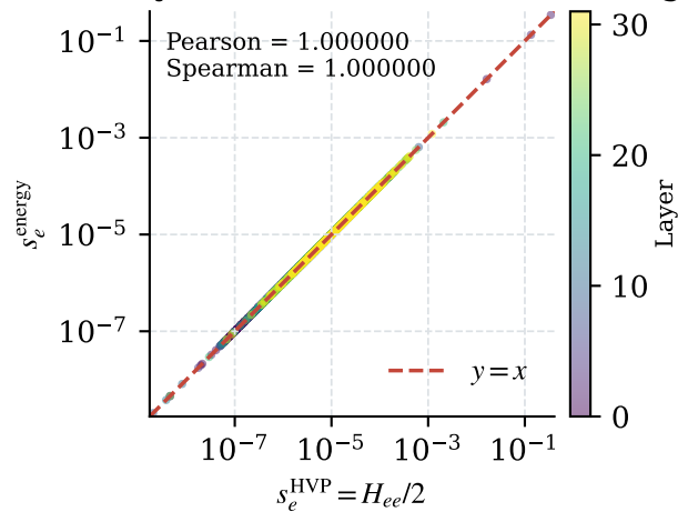
(a) Sanity check: HVP vs. Gram energy
