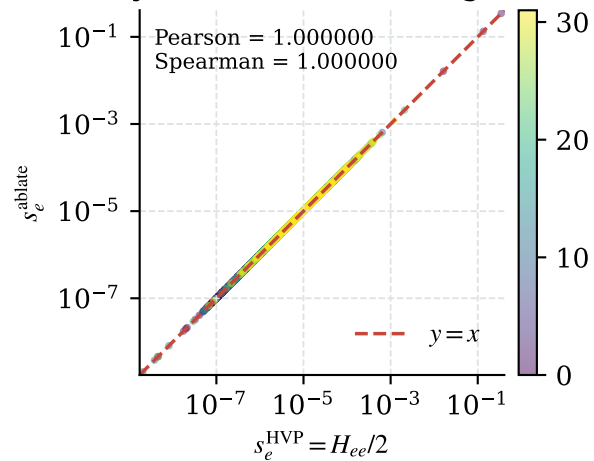
(b) Sanity check: HVP vs. single removal
