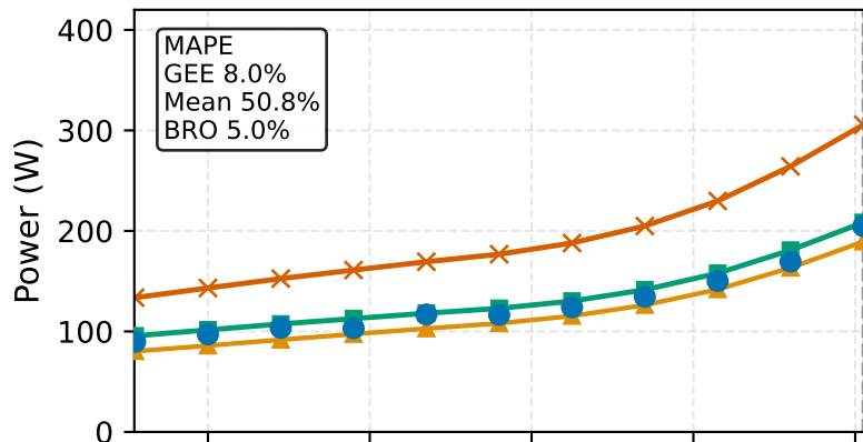
Qwen2, batch=1, seq=128
