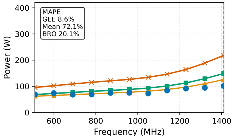
Qwen2, batch=1, seq=128
