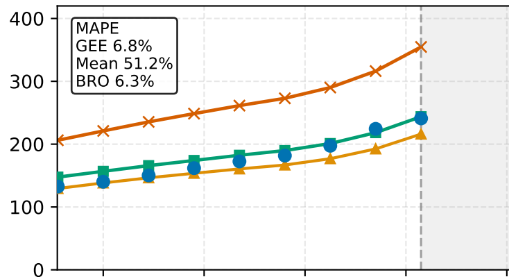
OPT, batch=8, seq=2048
