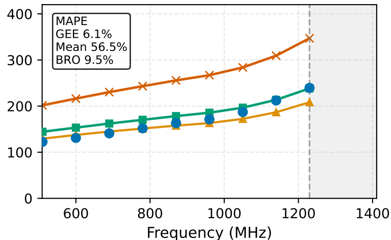
Qwen2, batch=1, seq=4096
