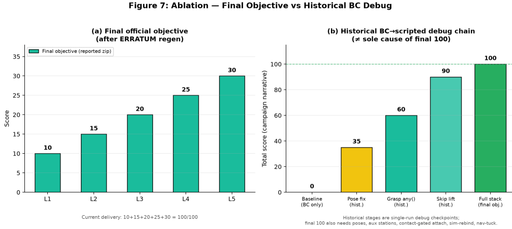
Figure 7: (a) Final official objective per level (reported zip). (b) Historical BC→scripted debug checkpoints from an earlier campaign—single-run narrative scores, not a claim that skip-lift alone yields 100 under current ERRATUM tasks. Interpret alongside Table 8: final delivery also required object-keyed poses, aux stations, contact-gated attach, sim-rebind, and nav-tuck.
