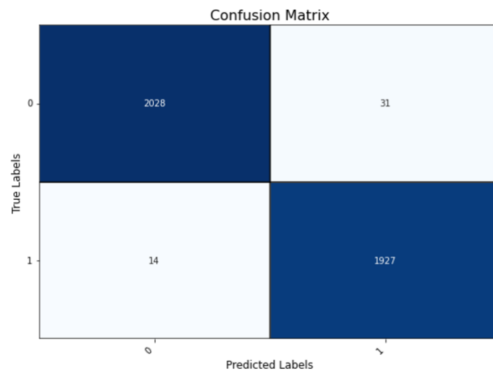
Figure 8: Confusion matrix for GB with the best parameters.
