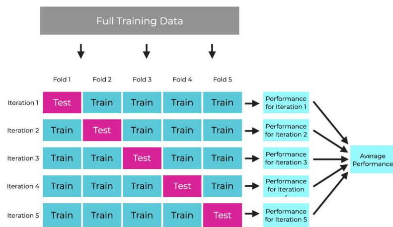
Figure 4: Visual representation of K-FOLD Cross Validation. [3]
