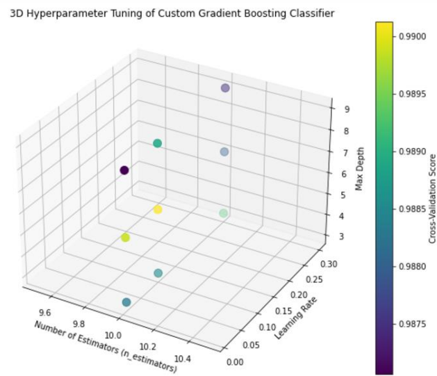
Figure 10: 3-D plot of Hyperparameter Tuning of GB where n_estimators is fixed and learning rate and max depth are the changing variables.
