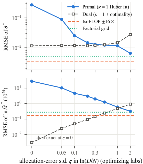
A. Precision against allocation error, same compute
