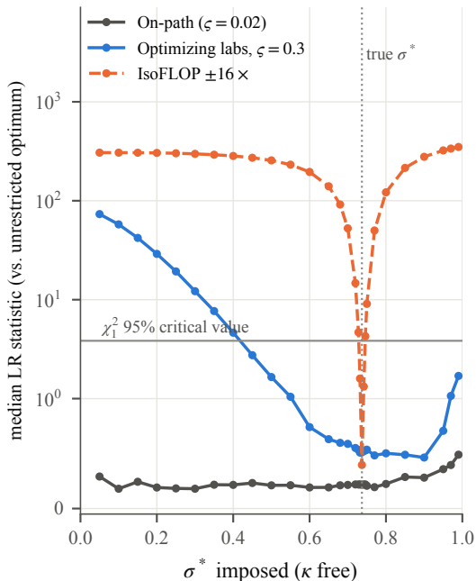
B. Profile likelihood of \sigma^* , \kappa free
