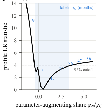
(c) Profile over the factor bias
