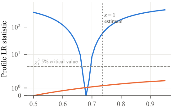
(a) Gaussian profile likelihood ratio
