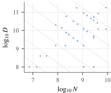
Muennighoff (1 epoch): sd = 1.97
