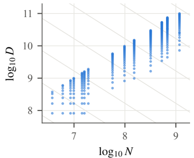
DataDecide (checkpoints): sd = 0.71
