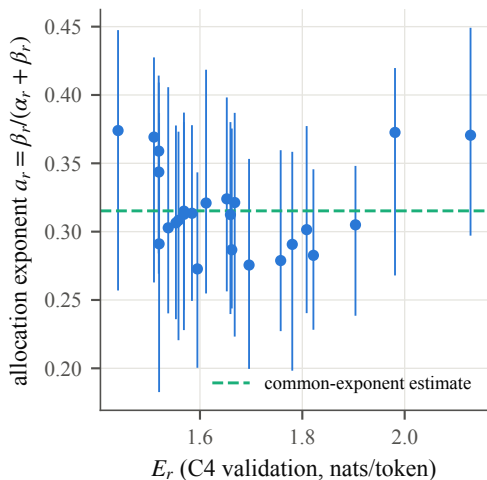
(b) DataDecide: separate fits by recipe
