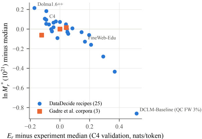
(a) Factor tilt of recipes (common exponents)
