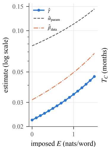
(b) Exponents rise with E ...
