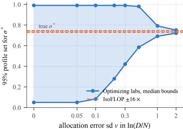
A. Median bounds of the set, \kappa free
