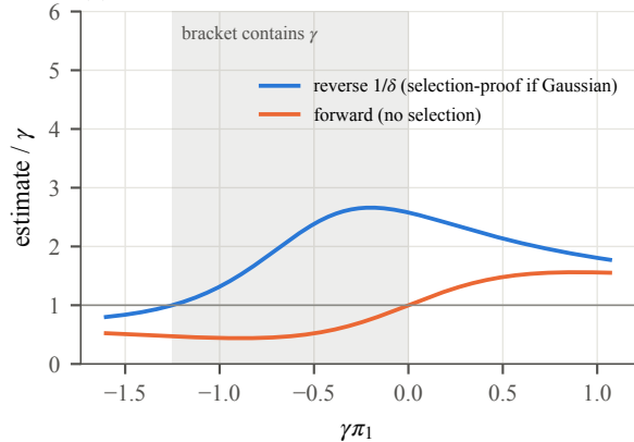
(b) Forward-reverse bounds
