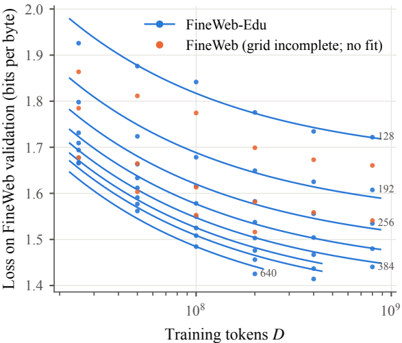
(a) Loss against data, by width
