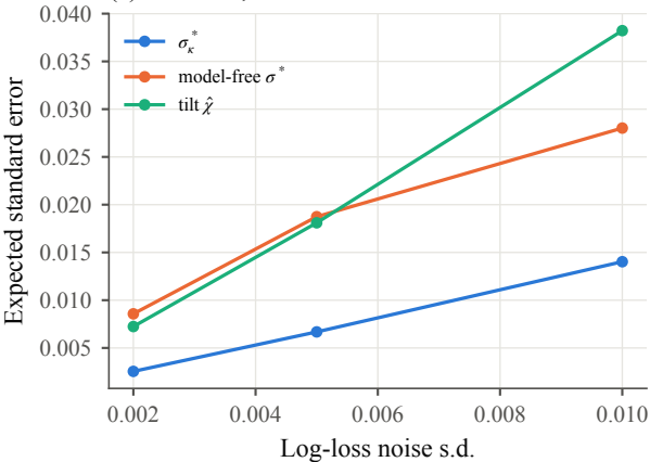
(a) Precision, convention P
