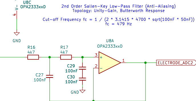
2nd Order Sallen–Key Low–Pass Filters
