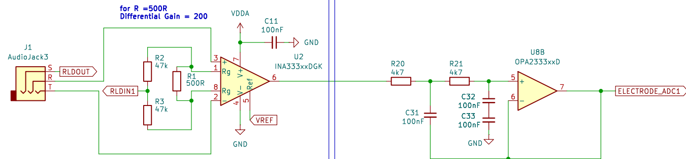
FIRST ELECTRODE JACK
