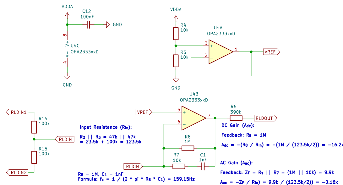
RIGHT LEG DRIVEN ELECTRODE NETWORK
