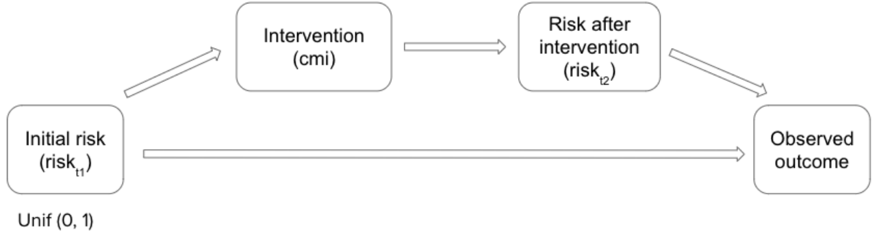
Figure 1: Causal diagram
