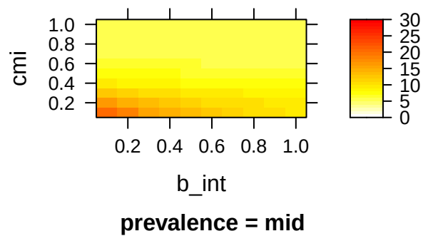
Mean Squared Error
