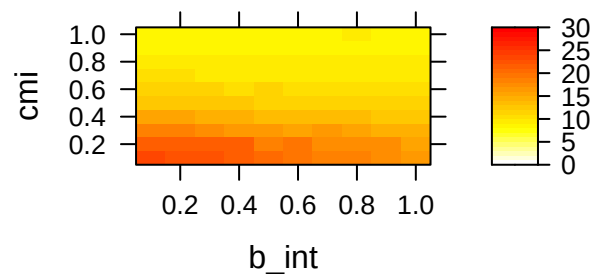
prevalence = high Mean Squared Error
