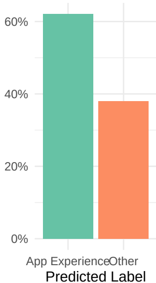
Classification Result
