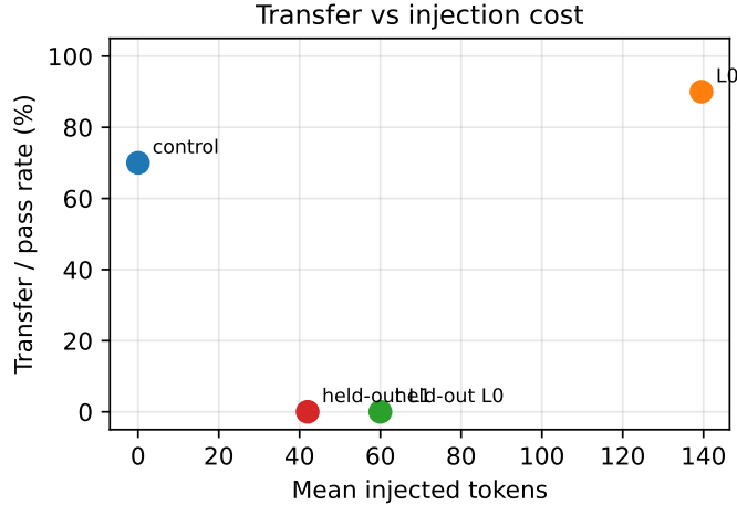
Figure 4: Transfer vs. injection cost on RMC-Bench core cases and held-out retention probe.
