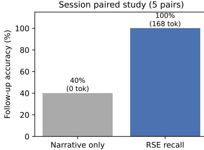
Figure 2: Session paired study: structured recall vs. narrative-only follow-up.
