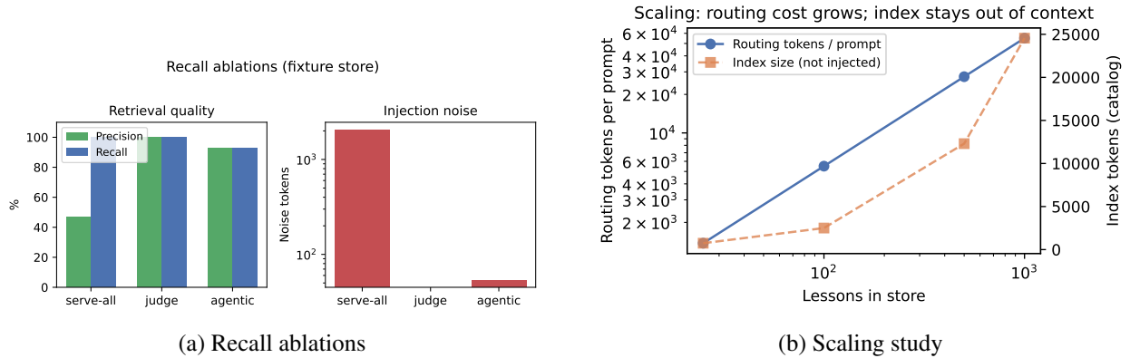
Figure 3: Retrieval filtering removes noise; routing cost scales with store size while index stays out of context.
