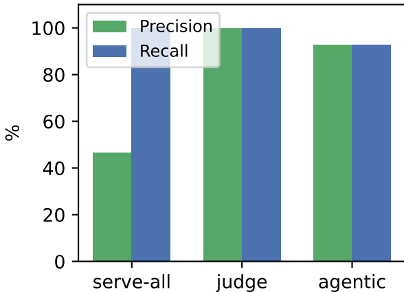
Retrieval quality
