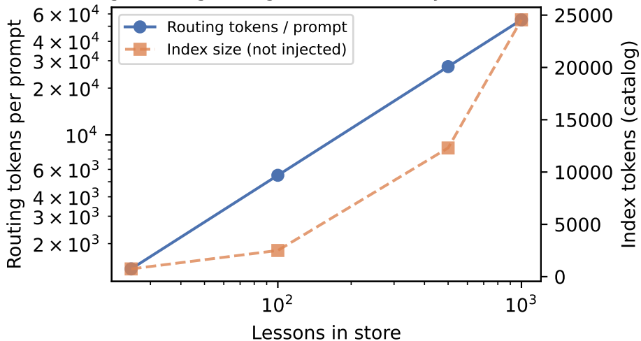
Scaling: routing cost grows; index stays out of context
